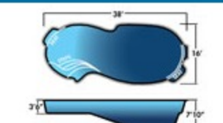
Dolphin II 16' x 38' x 7'10"
